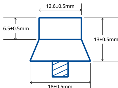
Figure 3: profile of football stud (new)
