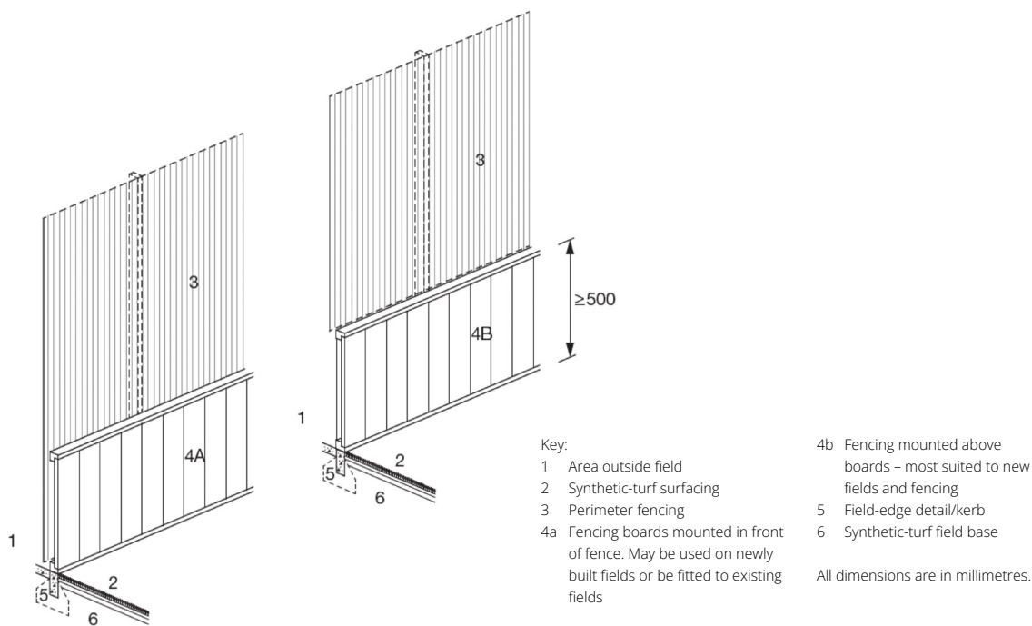
Figure 64: fencing panels used when the synthetic-turf surface is laid up to a fence
