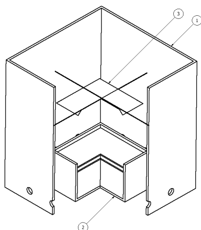
Figure 36: sectional schematic of apparatus for measuring heat (temperature increase)
