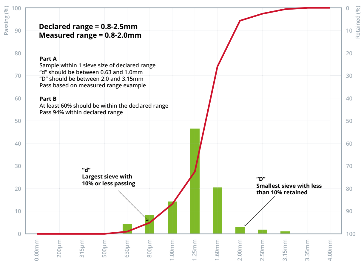
Figure 53: Example of particle distribution curve
