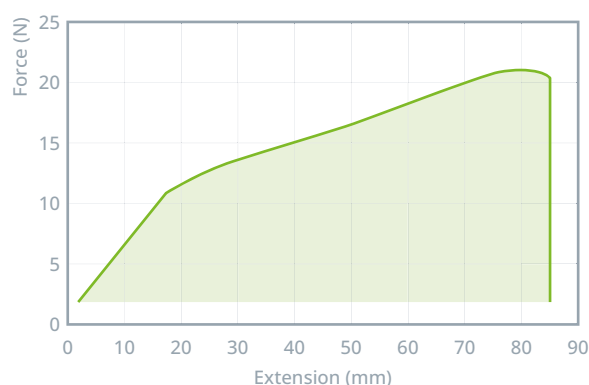
Figure 63: typical extension – force plot from yarn test. The area under the curve is the yarn energy absorption
