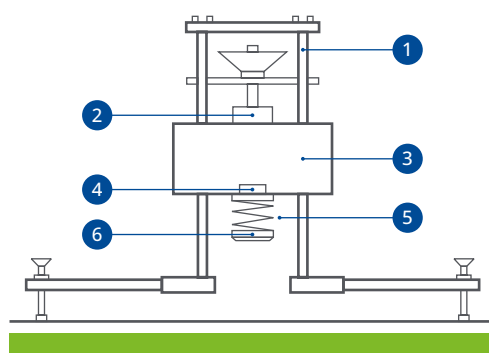
Figure 8: AAA test apparatus
