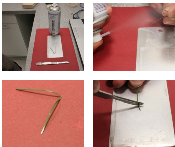
Figure 56: sample preparation procedure
