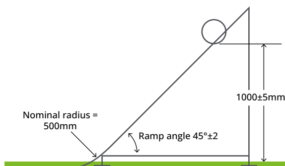
Figure 5: ball roll ramp
