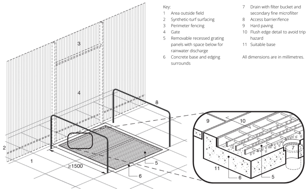
Figure 66: decontamination/boot-cleaning grate (located outside all entrances)
