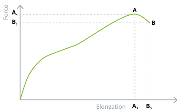
Figure 61: force-elongation graph from a tensile test
