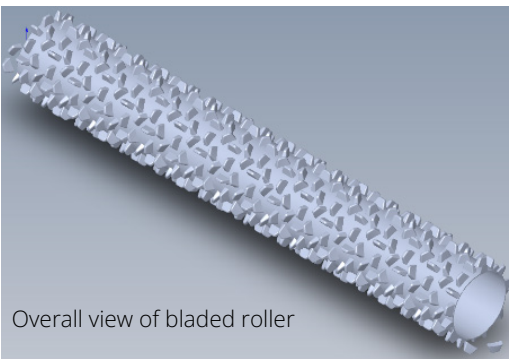
Figure 41: bladed roller
