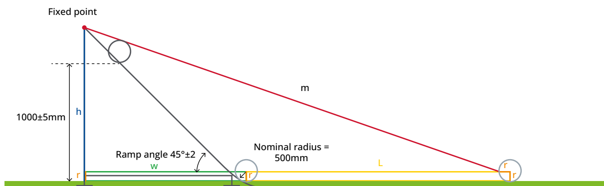
Figure 4a: additional ball roll length measurement procedure
