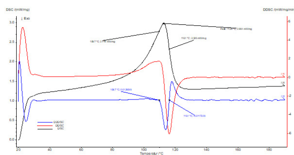
Figure 1: Example for peak (circled in Red). The 1st derivative at this point is 0.
