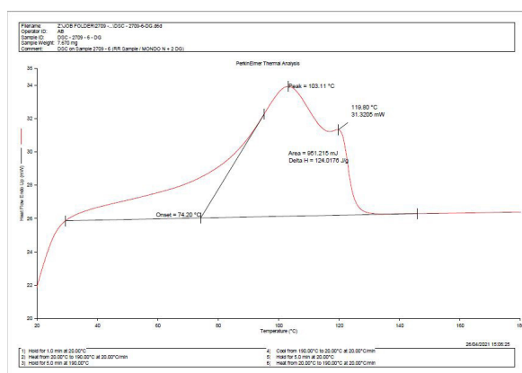
Figure 51: DSC curve representing melting behaviour of a fibre with a blend of polymers
