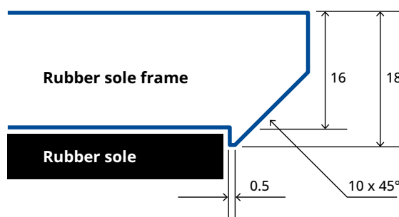
Figure 40: rubber sole configuration
