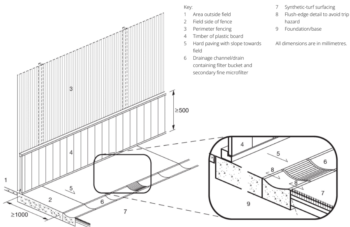
Figure 69: snow storage area
