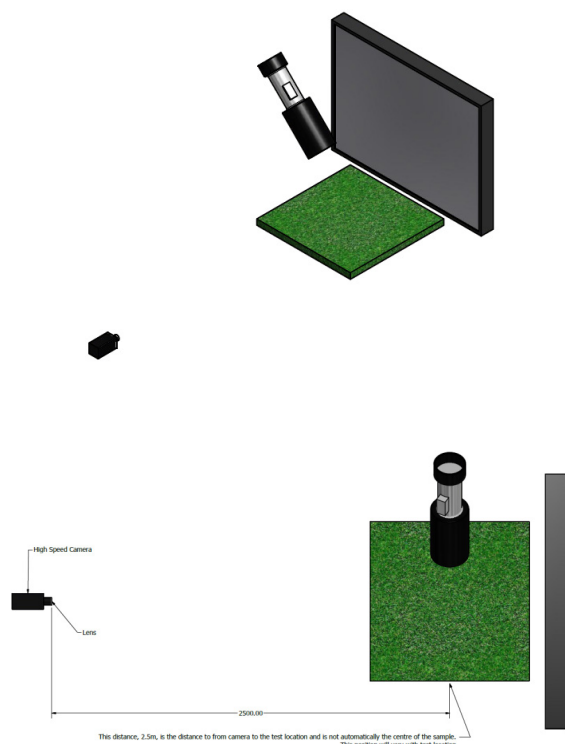
Figure 45: pictorial representation of the set-up
