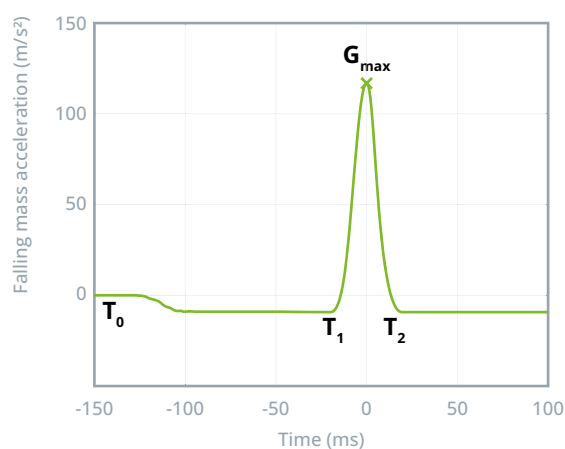
Figure 9: example of curve representing falling mass acceleration v. time
