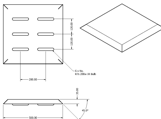
Figure 37: lamp and reflector arrangement
