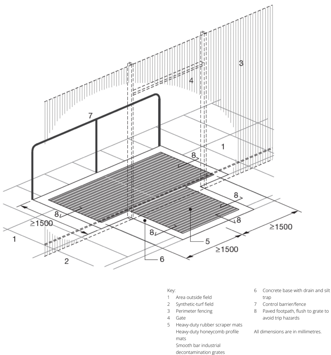
Figure 67: decontamination grate/boot cleaning – alternative configuration
