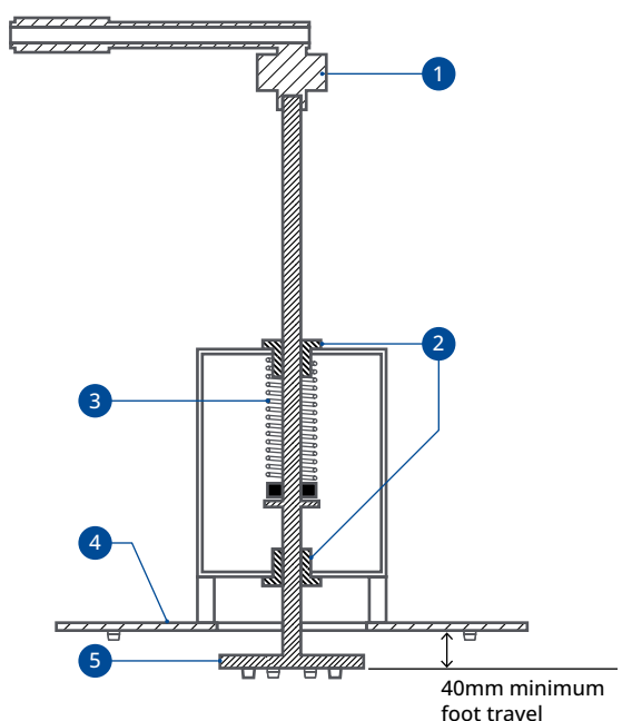
Figure 14: RTA apparatus
