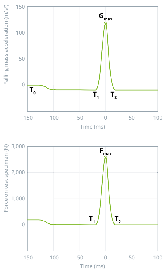
Figure 10: example curves showing falling mass acceleration v. time (top) and force on test specimen v. time (bottom)
