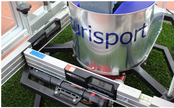
Figure 32: machine levelled
