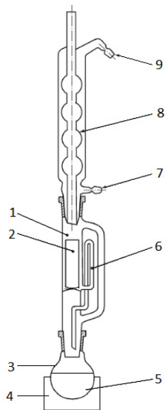
Figure 1: Soxhlet extractor
