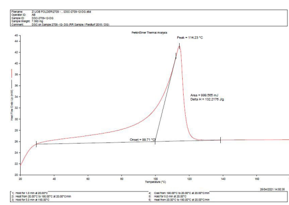
Figure 50: example of DSC curve with single melting peak
