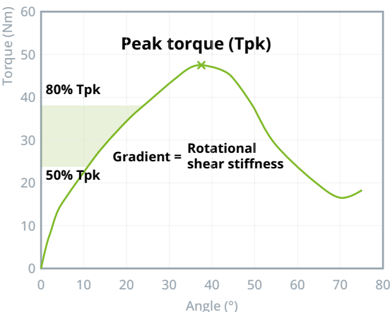
Figure 16: example plot of torque v. angle, illustrating the region used to calculate the rotational shear stiffness
