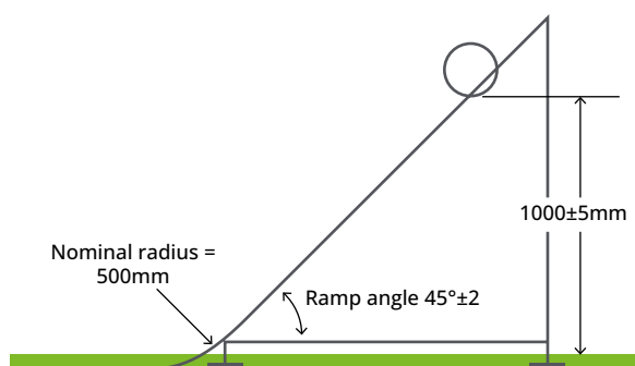
Figure 4: ball roll ramp
