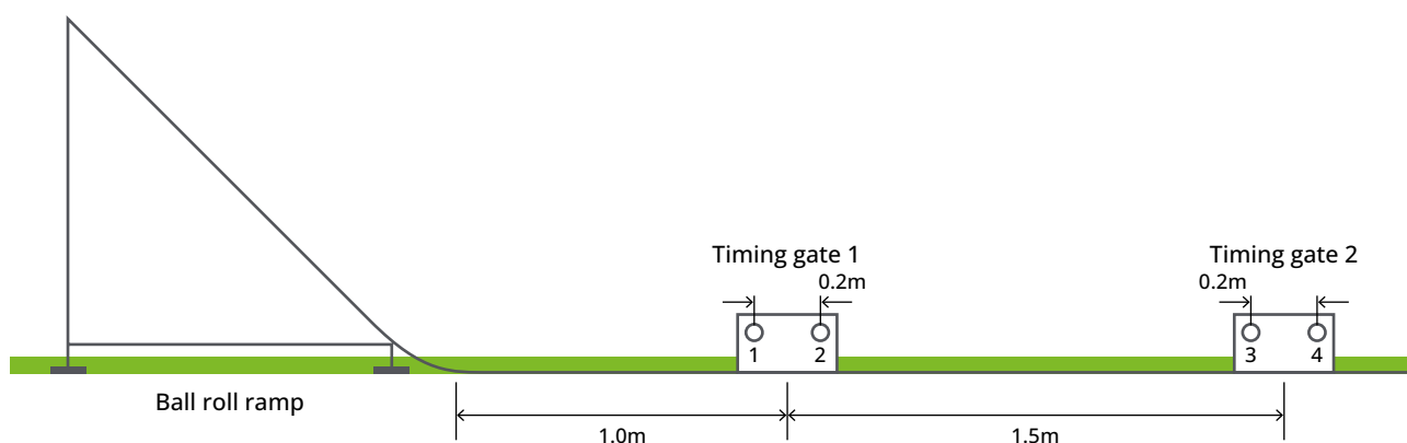
Figure 6: ball roll ramp and timing gate positions
