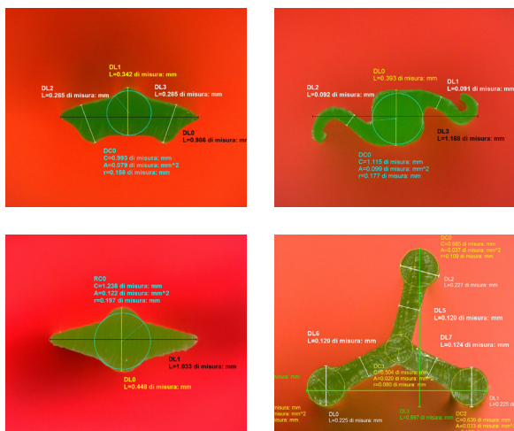
Figure 59: typical common fibre shapes
